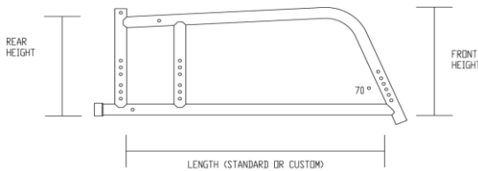
Frame Dimensions
