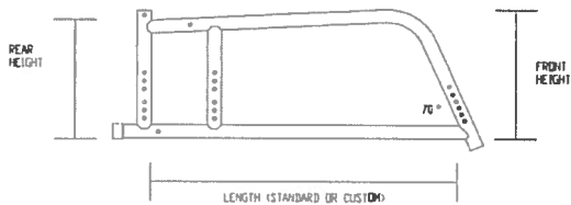
Frame Dimensions
