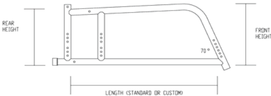
Frame Dimensions
